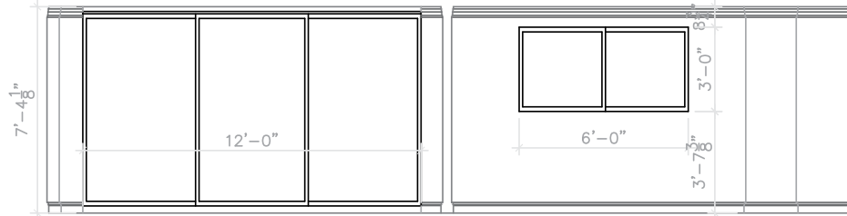
ROOM 821 ELEVATION 2
